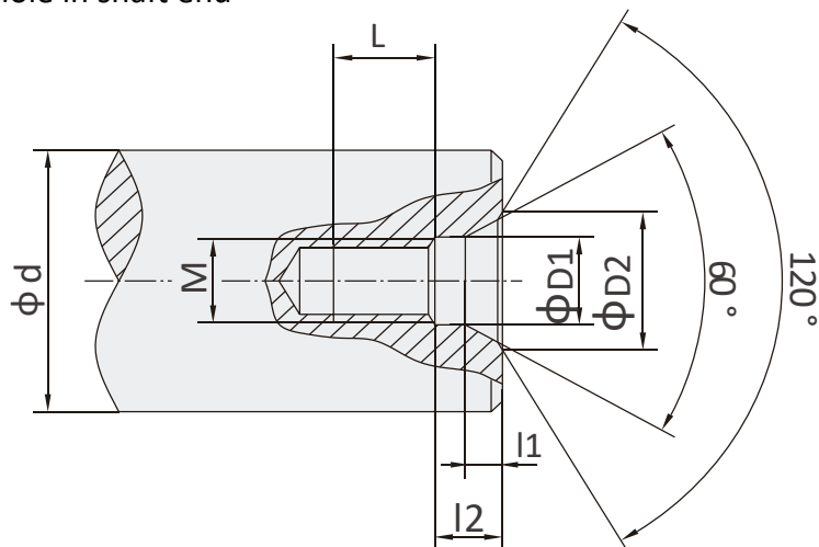
Type C screw central hole in shaft end
