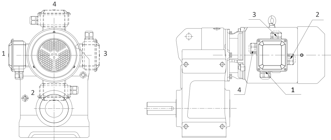
Motor terminal box and cable entry position ( View: Motor afterbody )
